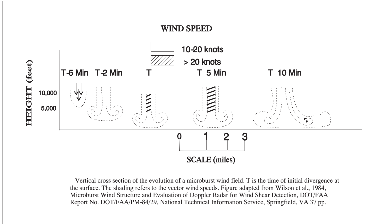
FIG 7-1-13 Evolution of a Microburst
