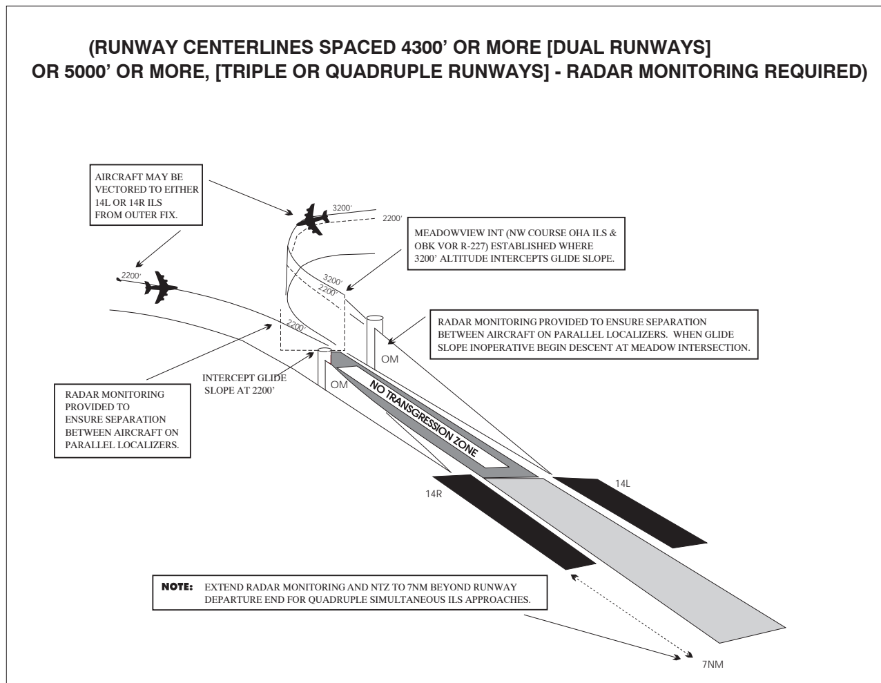
FIG 5-4-17 Simultaneous Parallel ILS Approaches
