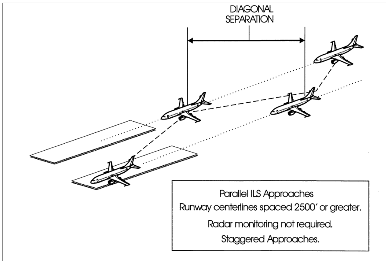
FIG 5-4-16 Staggered ILS Approaches
