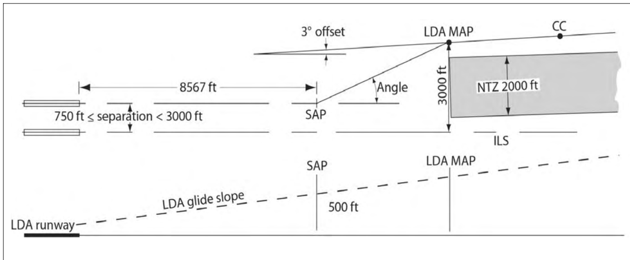
FIG 5-4-19 SOIA Approach Geometry
